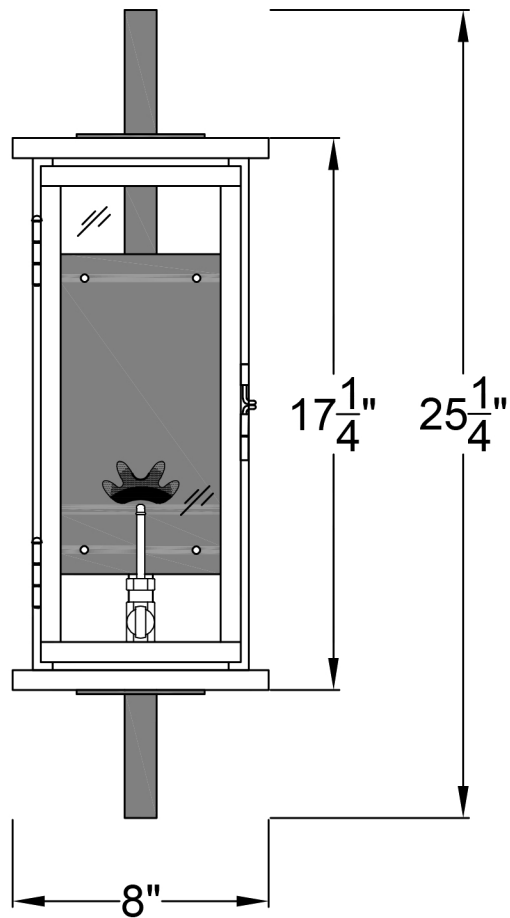
Front View
