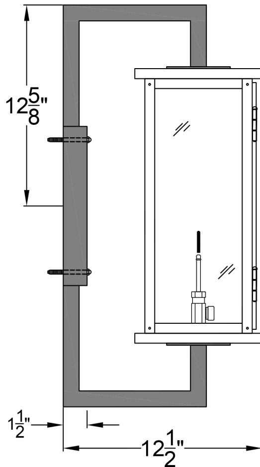
Side View
