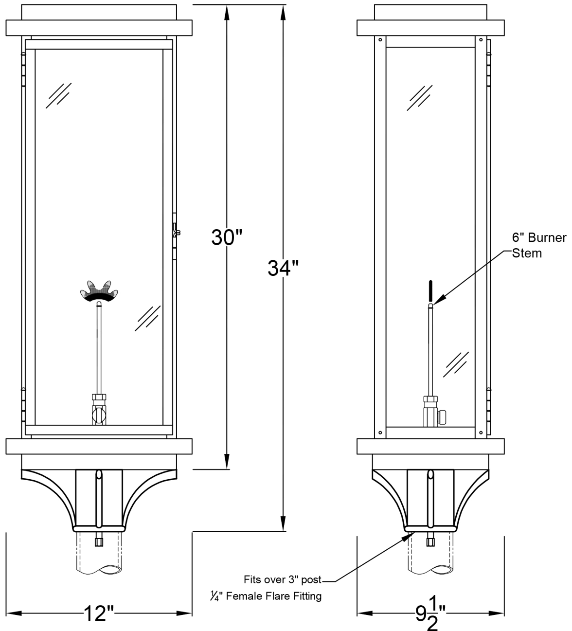
Front View
