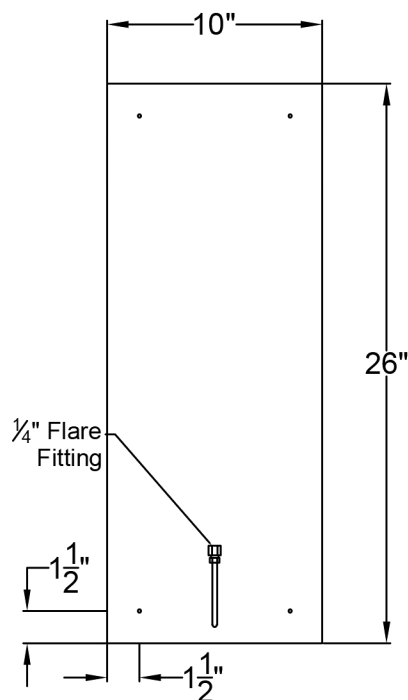
Backplate
