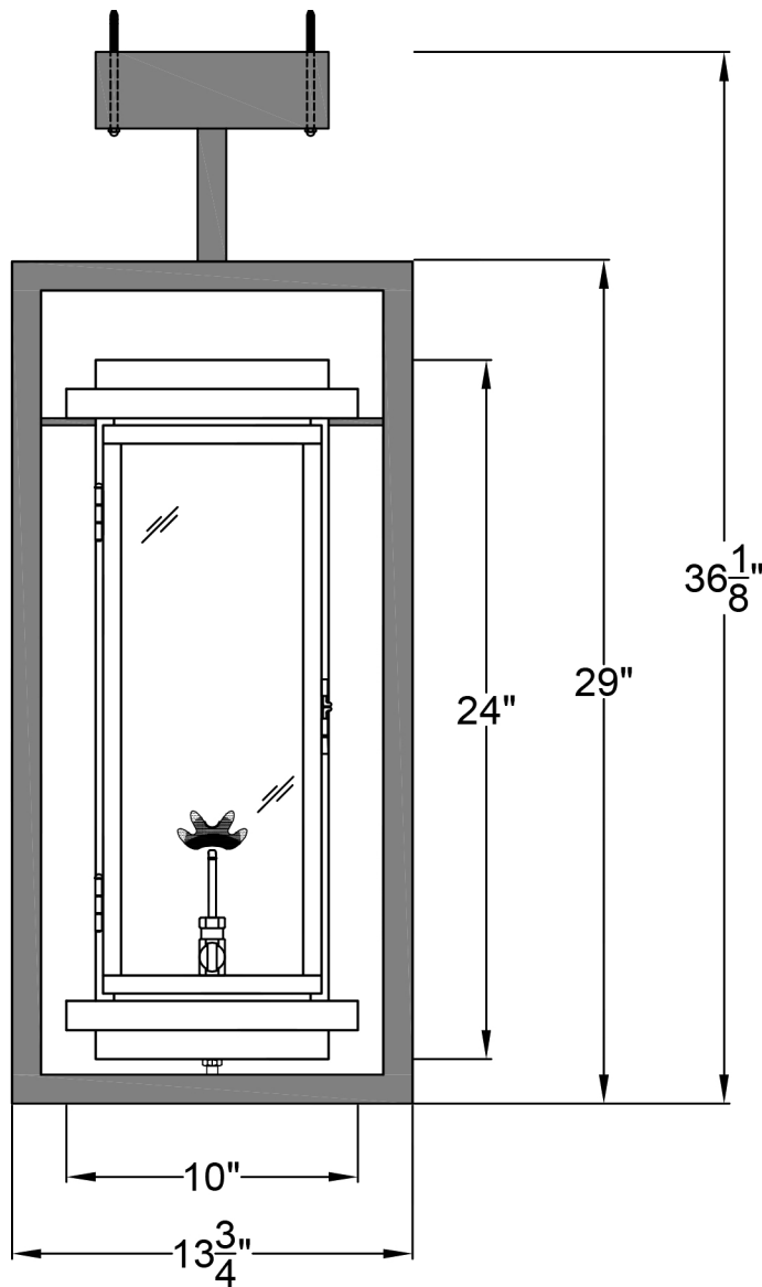
Front View
