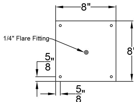
Ceiling Mount
