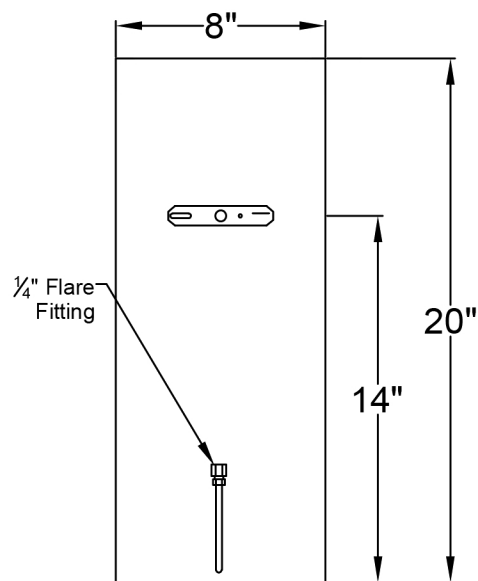
Backplate
