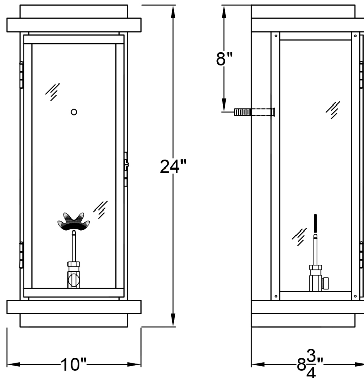
Front View
