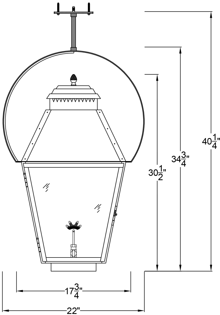
Front View
