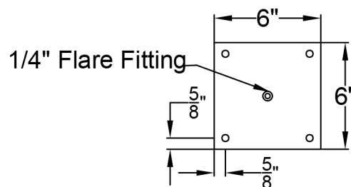
Ceiling Mount
