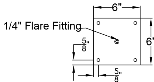
Ceiling Mount
