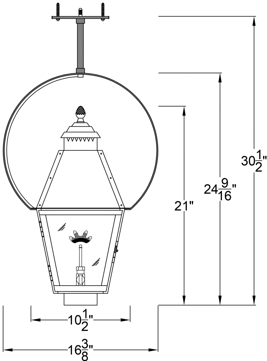
Front View
