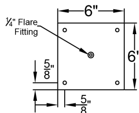
Ceiling Mount
