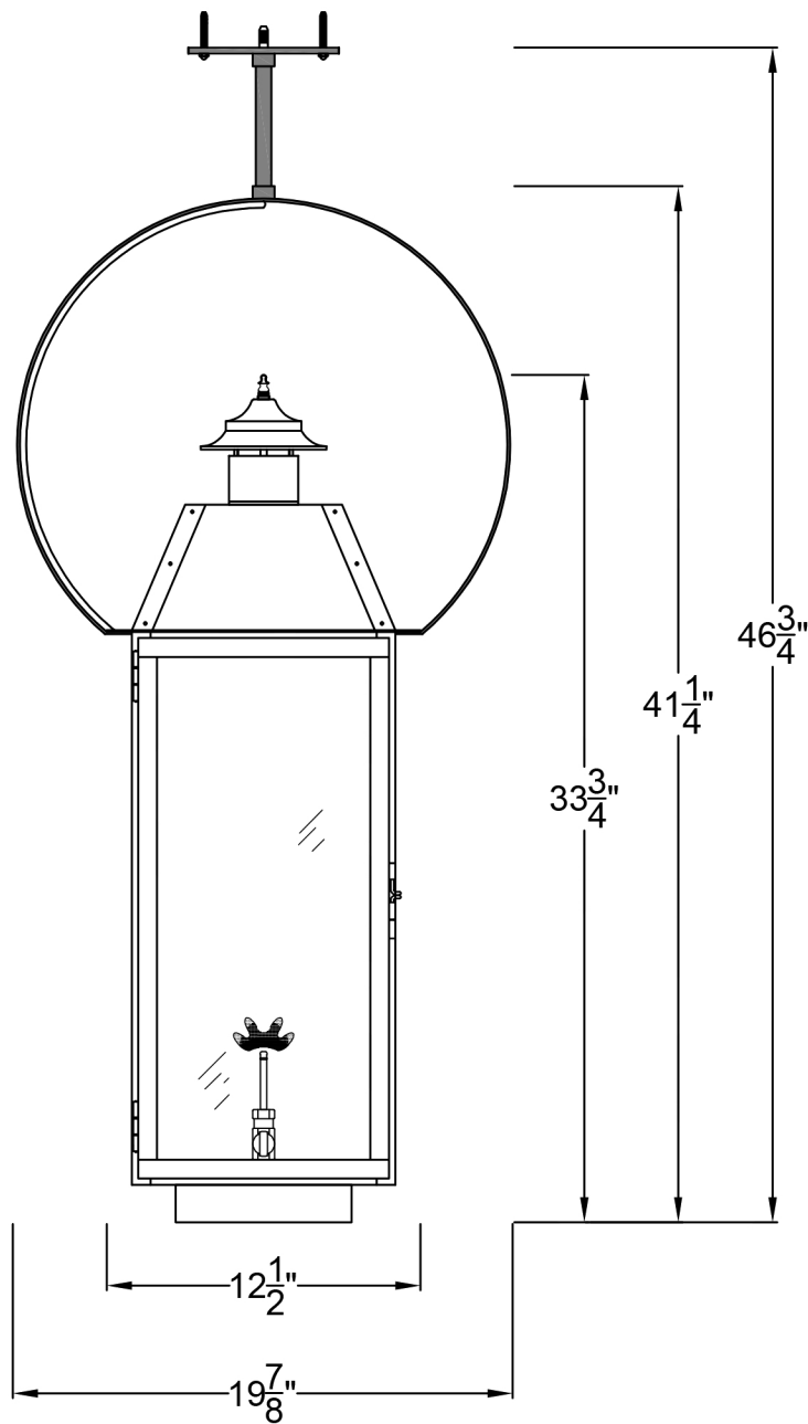
Front View
