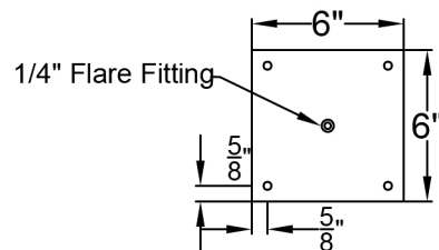
Ceiling Mount
