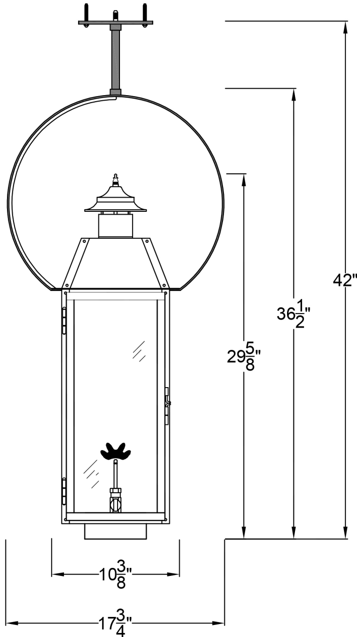
Front View
