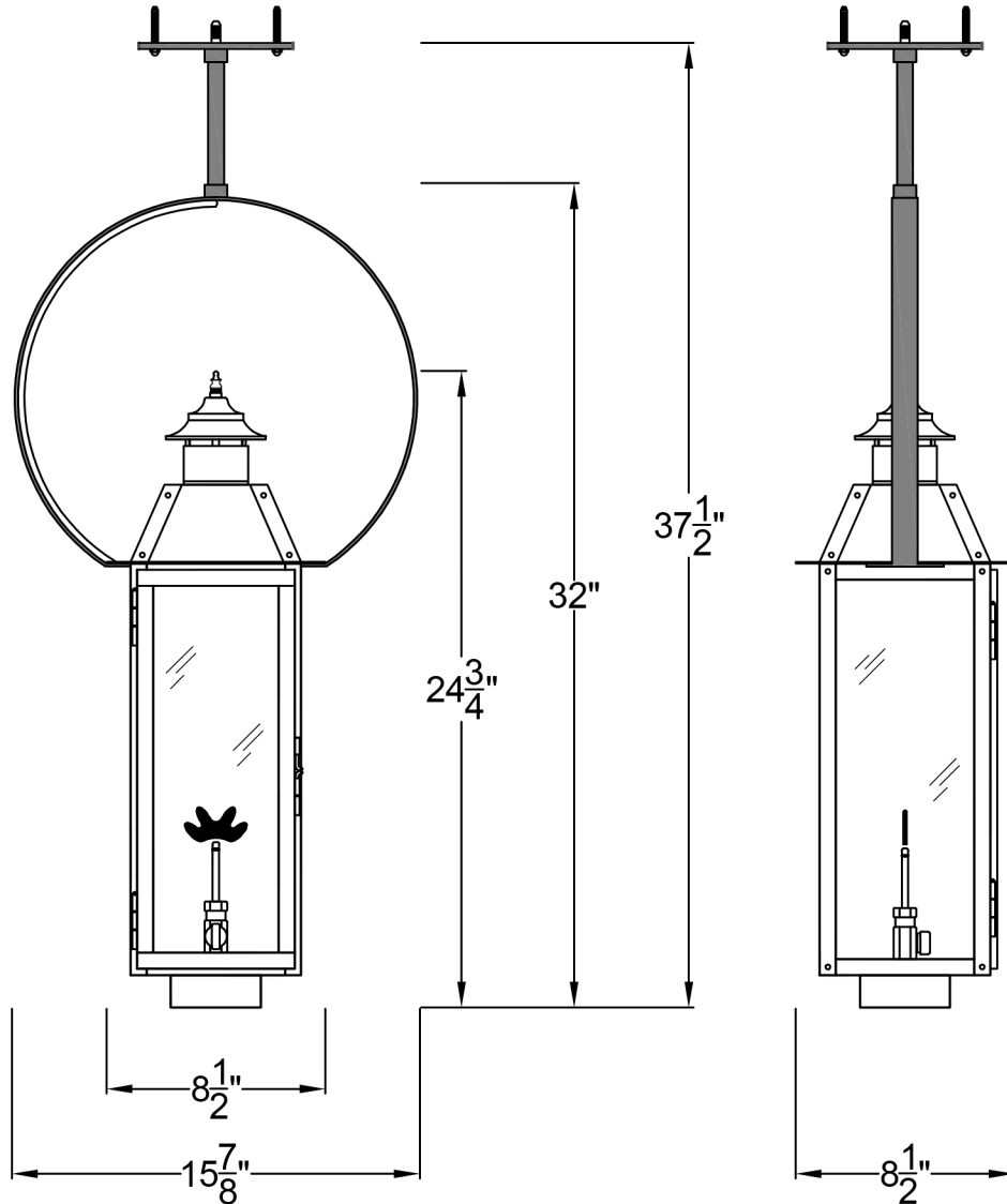
Front View
