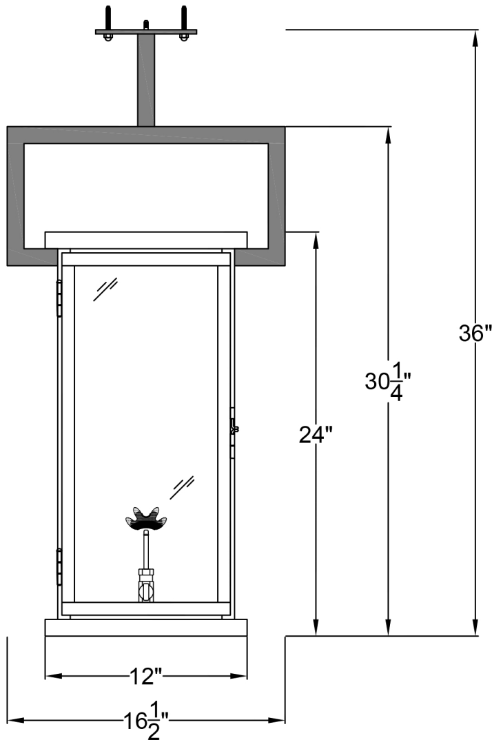
Front View
