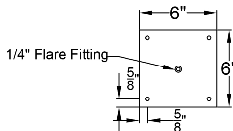
Ceiling Mount
