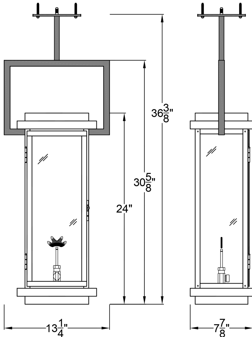
Front View
